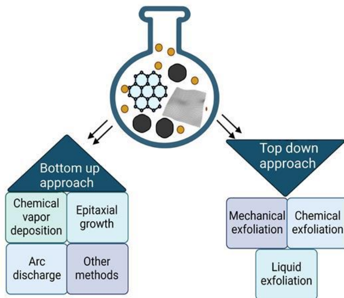
Figure 3. Synthesis approaches for graphene and its derivatives.
