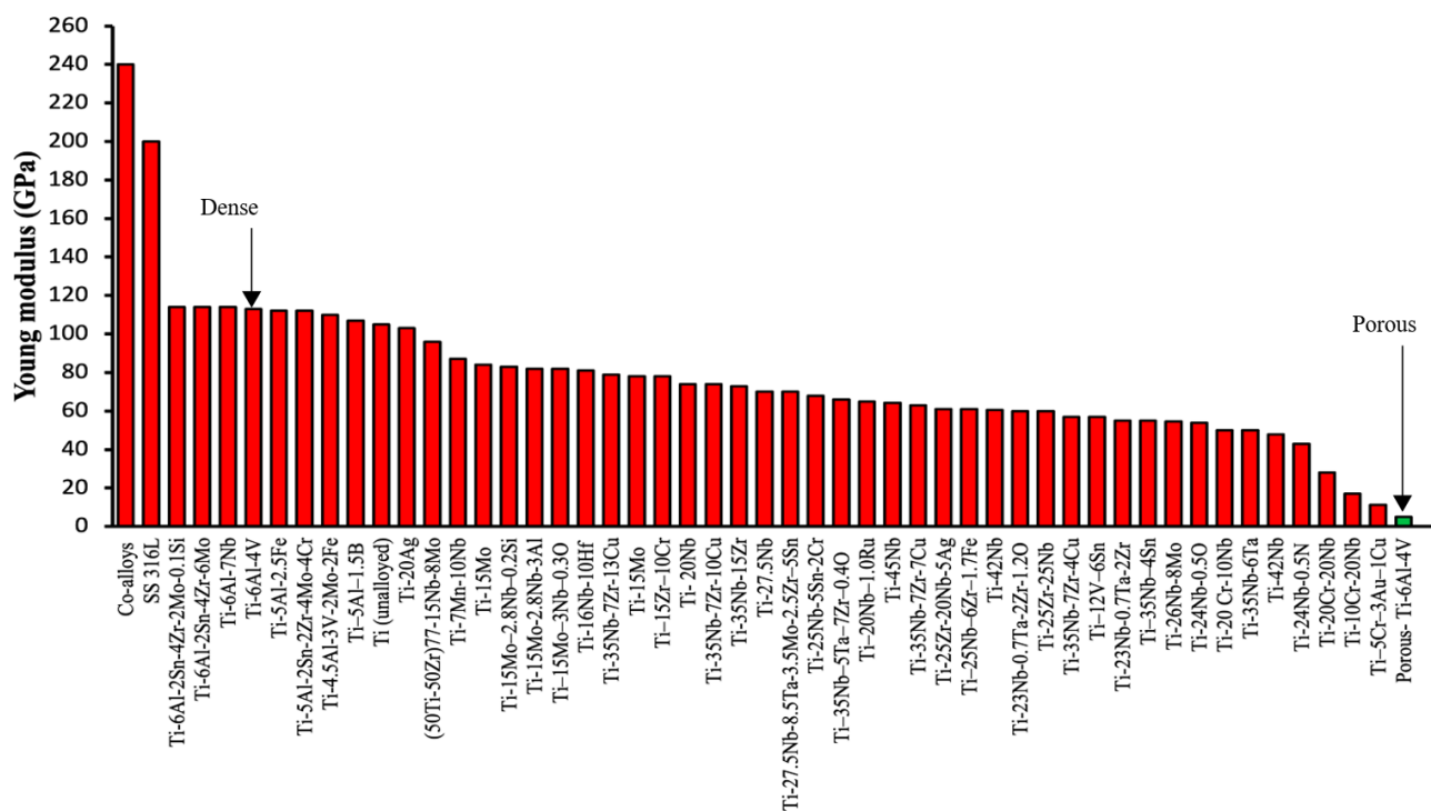
Figure 2. Elasticity modulus of various dense Ti alloys with a comparison of porous Ti-6Al-4V.
